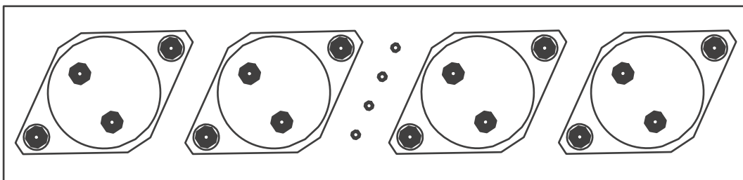
TEMPLATE FOR DRILLING HEAT SINKS FOR OUTPUT TRANSISTORS AND BIAS DIODES
